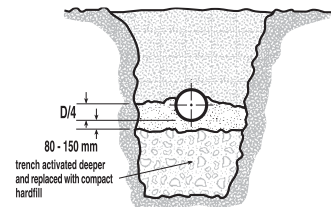
TRENCH IN POOR FOUNDATION SITUATION
